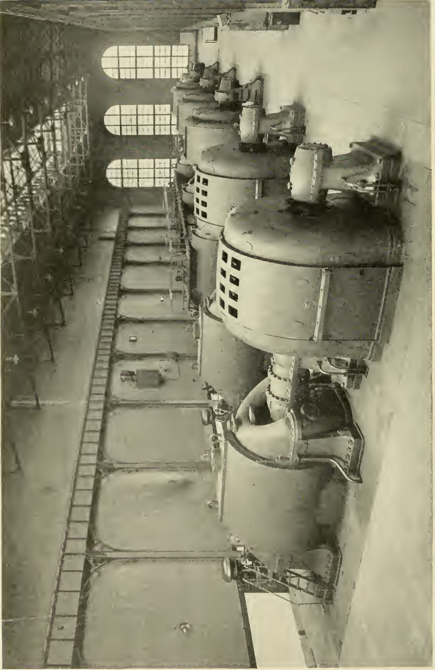
WESTINGHOUSE-PARSONS TURBOGENERATORS, EACH OF 5500-K.W. CAPACITY, INSTALLED FOR THE PENNSYLVANIA TUNNEL AND TERMINAL COMPANY, LONG ISLAND
